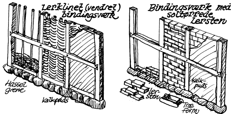
FIG 7: Timber frame infillings. Left: Wattle and daub. Right: Sundried and unburnt clay bricks. Both finished with lime plaster and lime wash. Drawing: Søren Vadstrup
