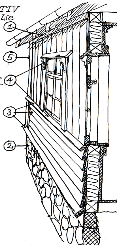
FIG 5: Typical Wooden Claddings of Timber Frame Buildings in Denmark, and the affiliated details in corners and around windows etc. (Drawing: Søren Vadstrup). The technical names are in Danish, but both in English and Russian the names of similar constructions and details can be find.
